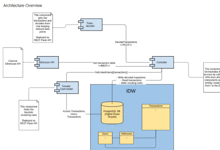
Figure 5. Showing the Intelligence Data Warehouse Architecture, with data types, storage method, providers and microprocessors clearly identified.
