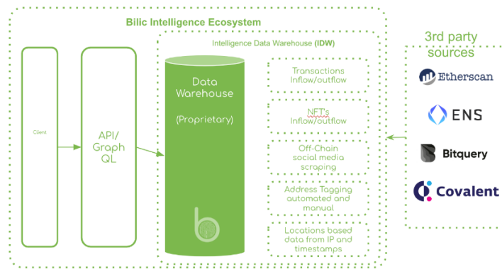
Figure 4. Showing the Intelligence Data Warehouse Architecture, with data types, storage method, providers and microprocessors clearly identified.
