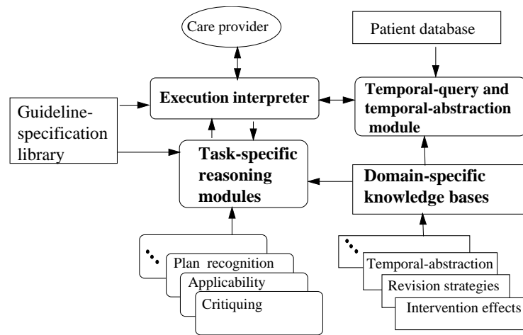
Figure 2.2 The guideline-support architecture. Arrows denote data or knowledge flow.
