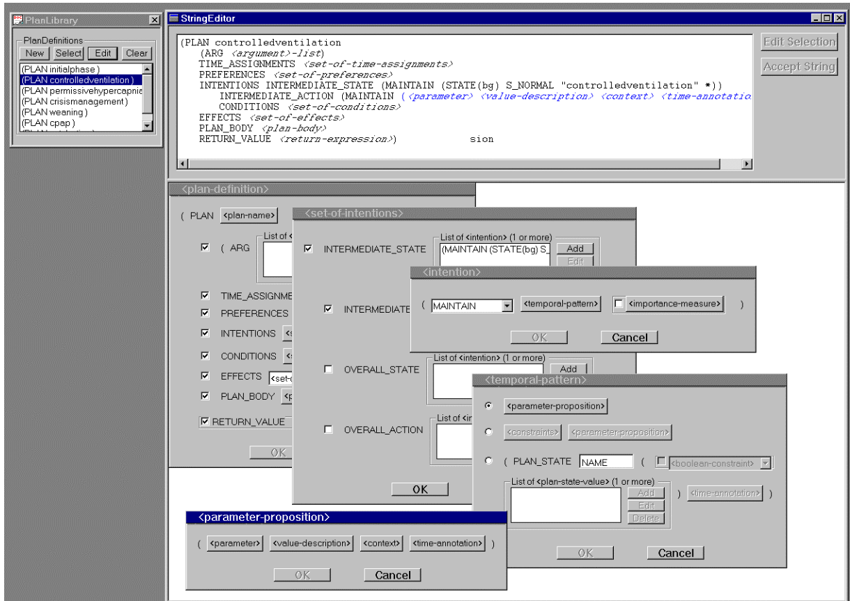
Figure 2.9 The string editor. The screen shot is showing acquisition of part of a treatment guideline for newborn infants who are being mechanically ventilated from a domain expert. In the string editor, the acquisition process is guided directly by the Asbru language's BNF syntax.
