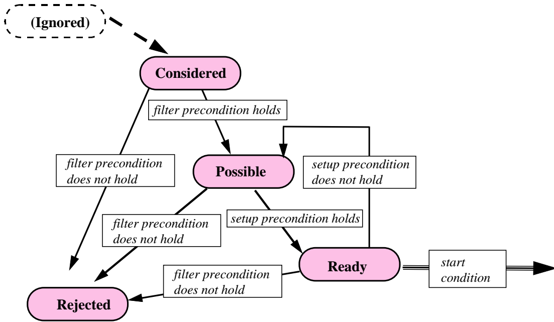
Figure 2.4 Plan-selection states and their state-transition conditions in Asbru. These states are relevant to library plans that are considered for execution.
