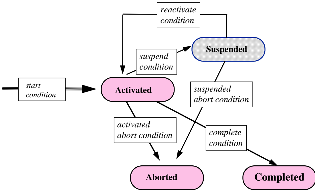
Figure 2.5 Plan-execution states and their state-transition conditions in Asbru. These states are relevant to instances of library plans that are being executed.
