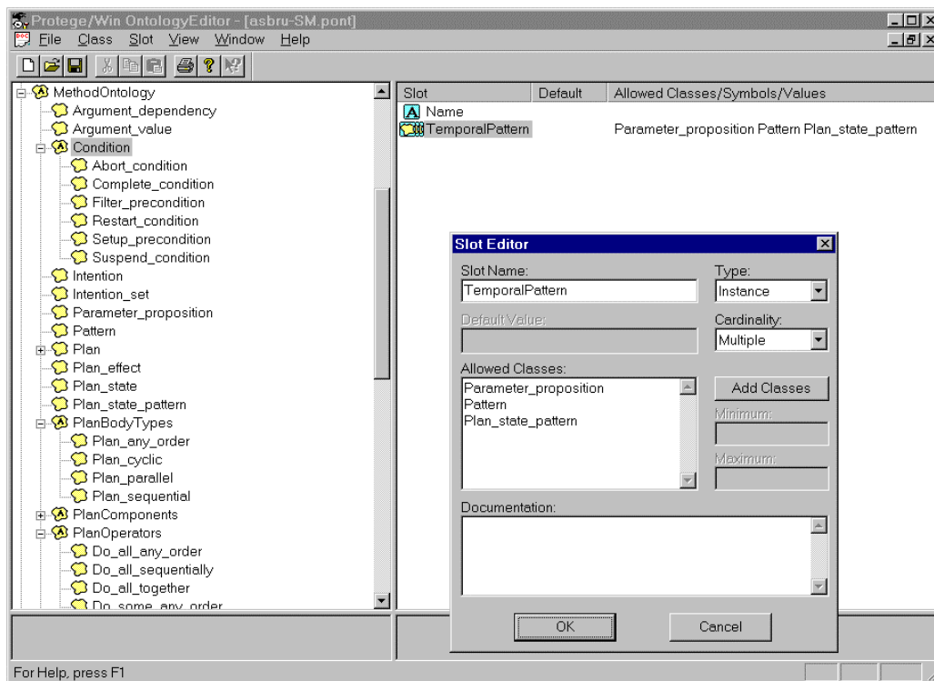
Figure 2.7 Part of the execution-support methods ontology, represented by the PROTÉGÉ/Win Ontology Editor.
