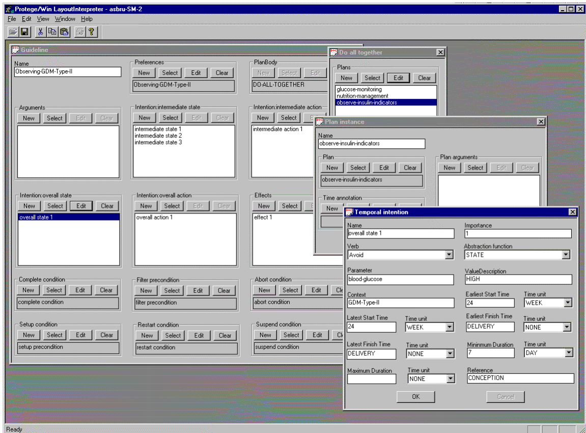
Figure 2.8 The Asbru knowledge-acquisition tool. The screen shot demonstrates acquisition of part of the gestational diabetes mellitus (GDM) type II guideline from a domain expert. The main window shows the guideline's components and is generated automatically by the Protégé/Win tools from an Asbru ontology. Two of the three subwindows show acquisition of one of three parallel (do-all-together) plans that the GDM guideline is composed of; the third shows a definition of the GDM guideline's overall state intention.
