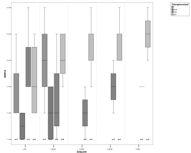
Figure 3. Sample of EDA: Boxplots (Printout Material)
