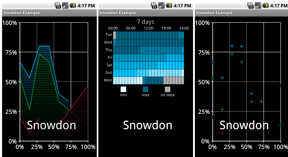
Figure 4.7: Line chart, heat map and scatter chart generated using Snowdon [Snowdon, 2015]
